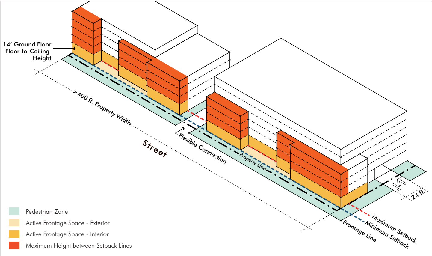
DRAFT Building Frontage Standards FIGURE 3-3
