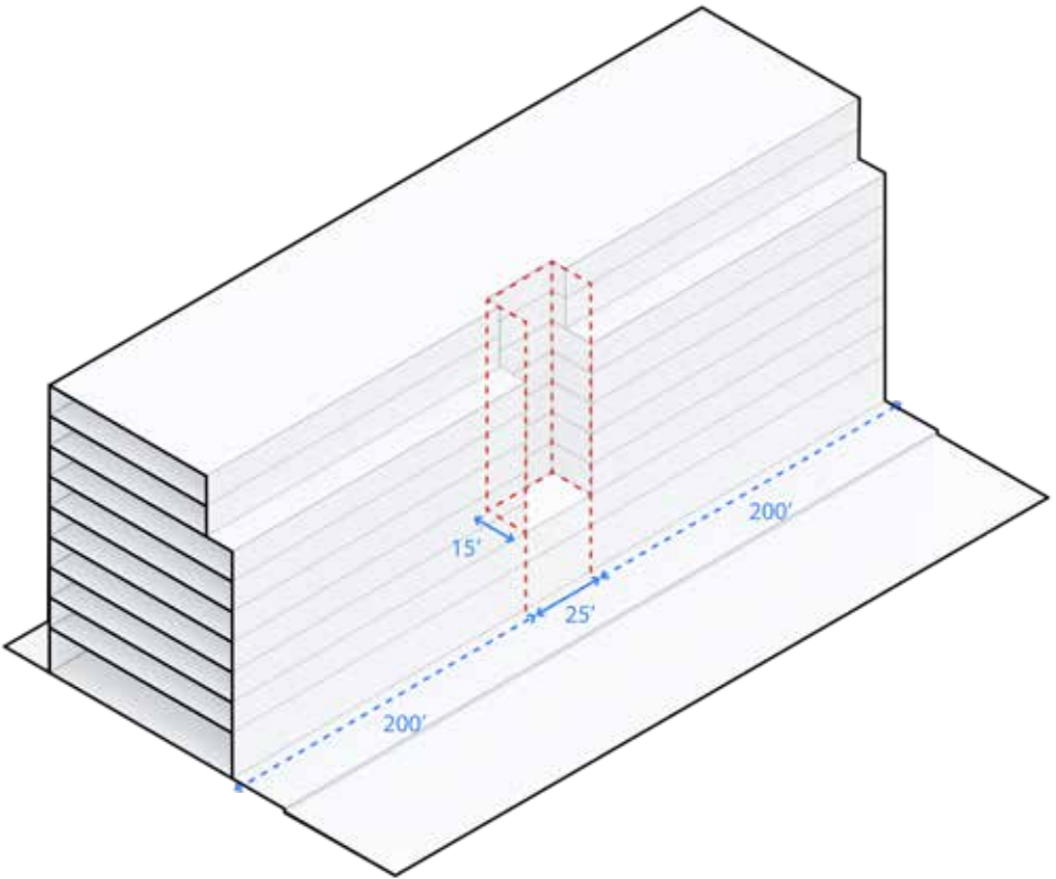
Figure 8.5.10 Example building massing breaks
