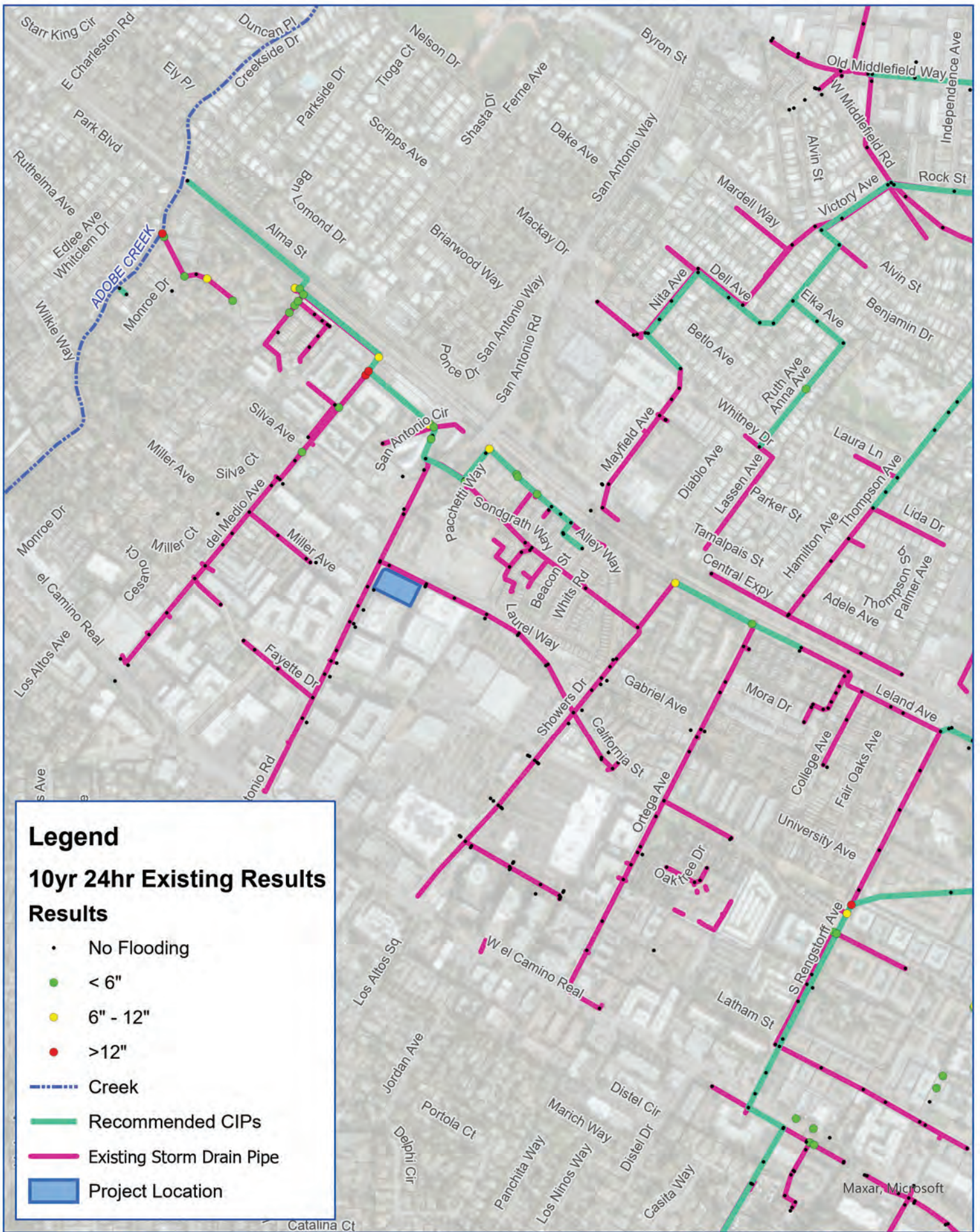
FIGURE 14: Storm Drain Existing 10yr Results
