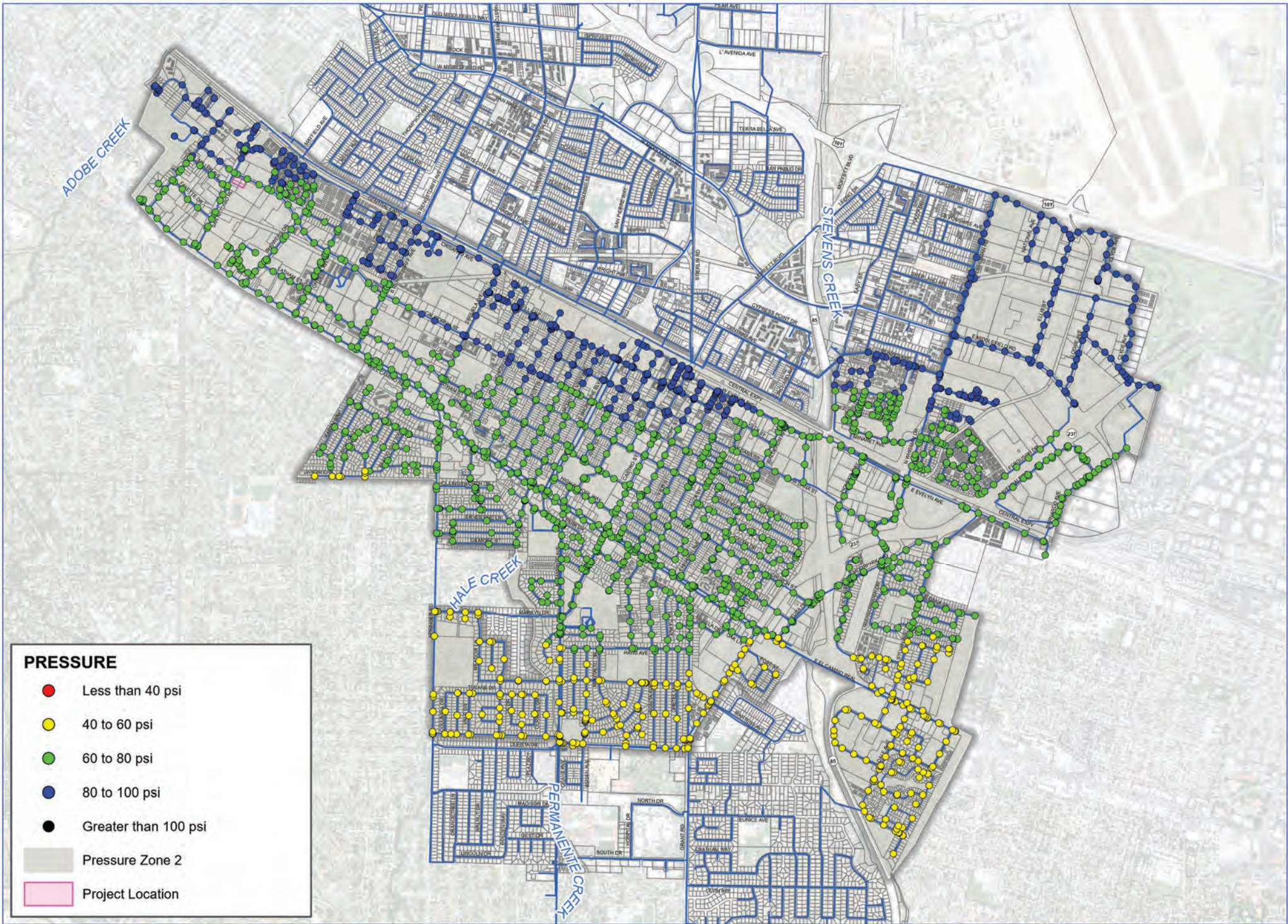
Peak Hour Demand (PHD) with Project Water System Model - Future Condition
