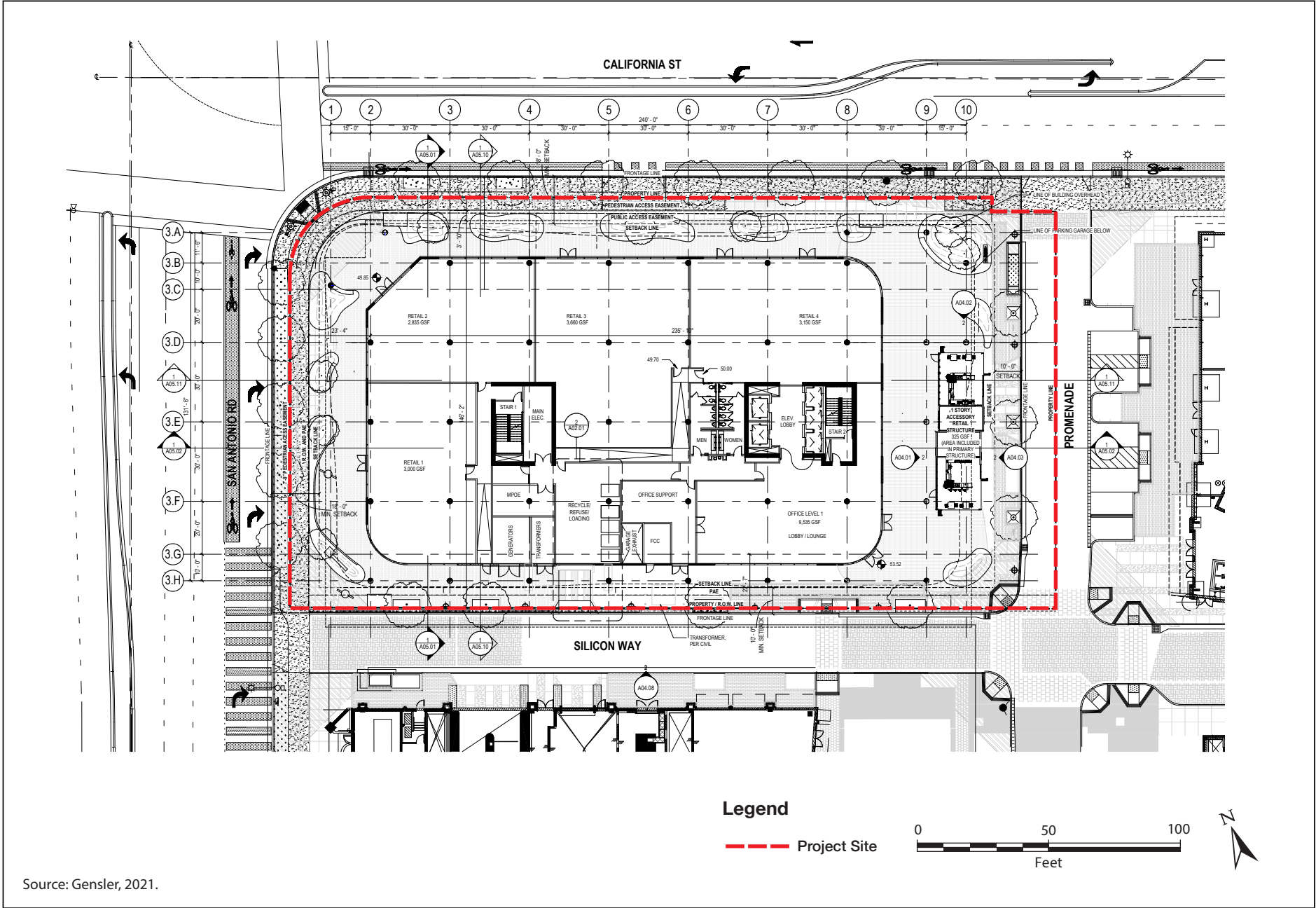
Figure 2-5 Site Plan—Level 1 San Antonio Phase III
