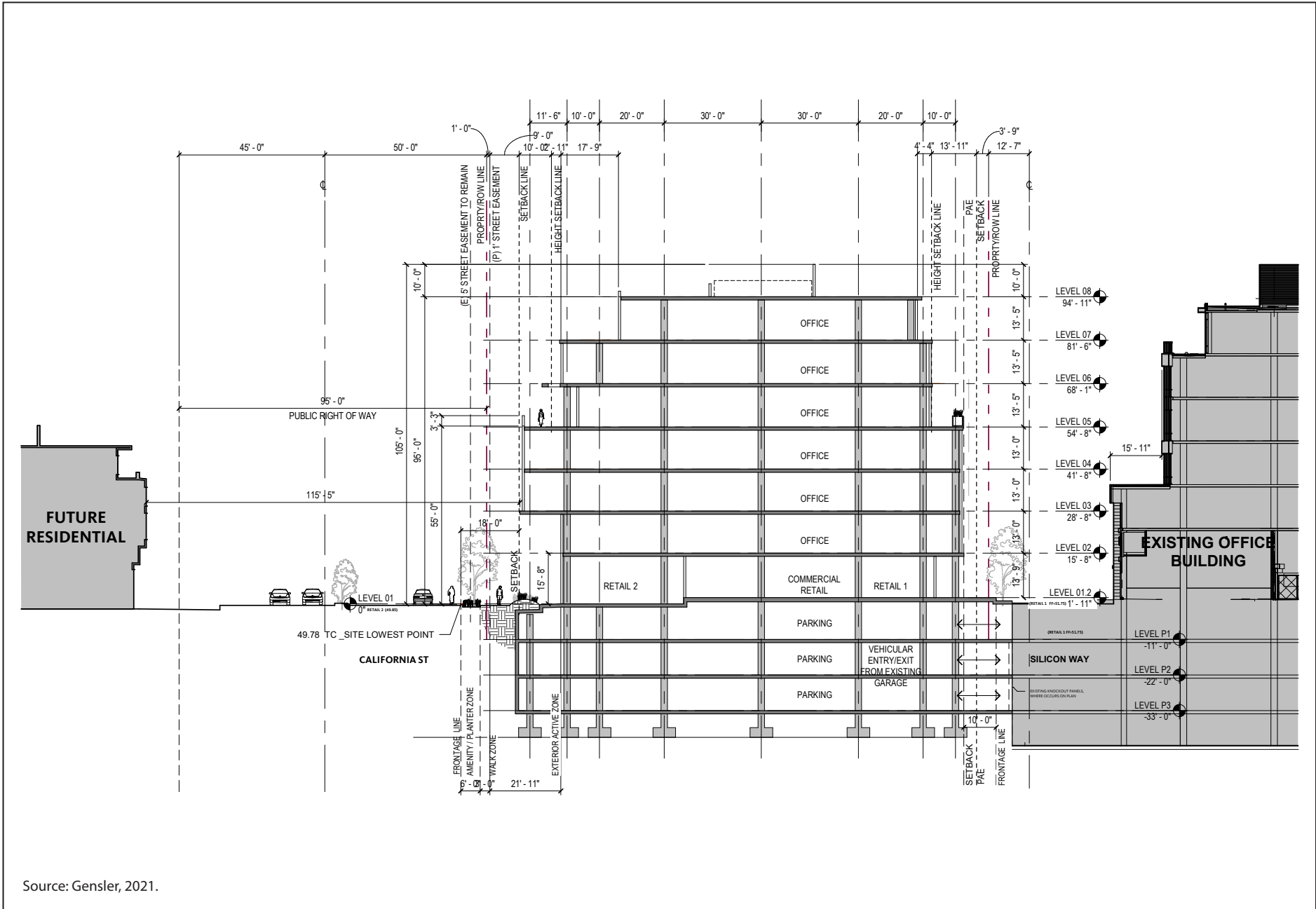
Figure 2-4 Proposed Site Cross-Section San Antonio Phase III
