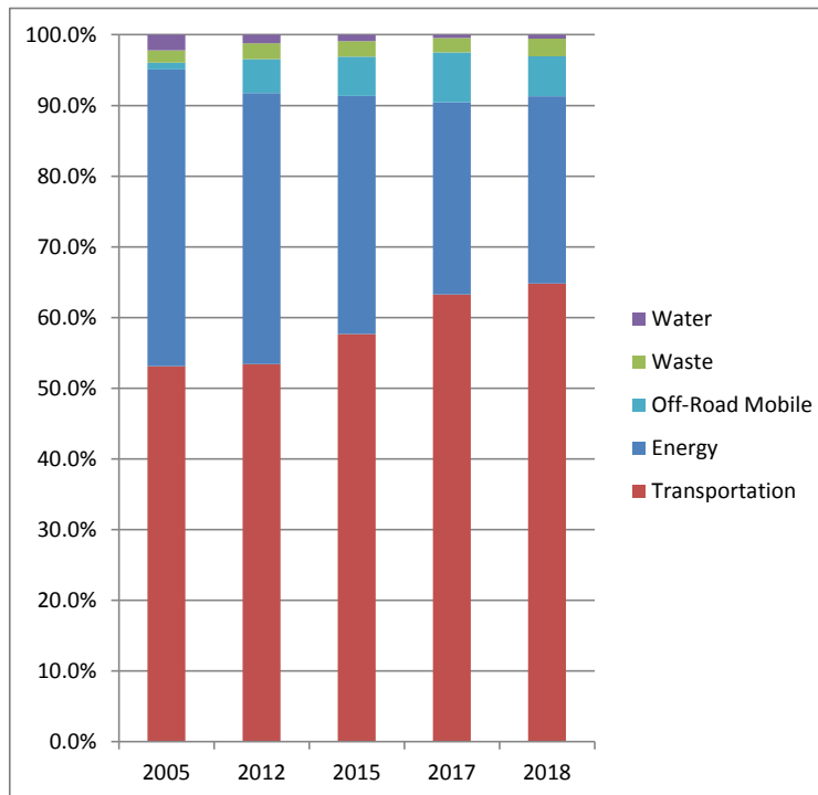
Percent of Total Emissions by Sector and Subsector, 2005-2018
