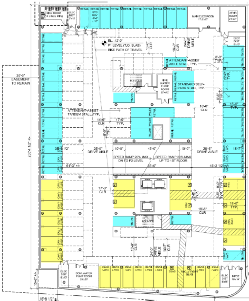
Figure 22. B1 Level Plan
