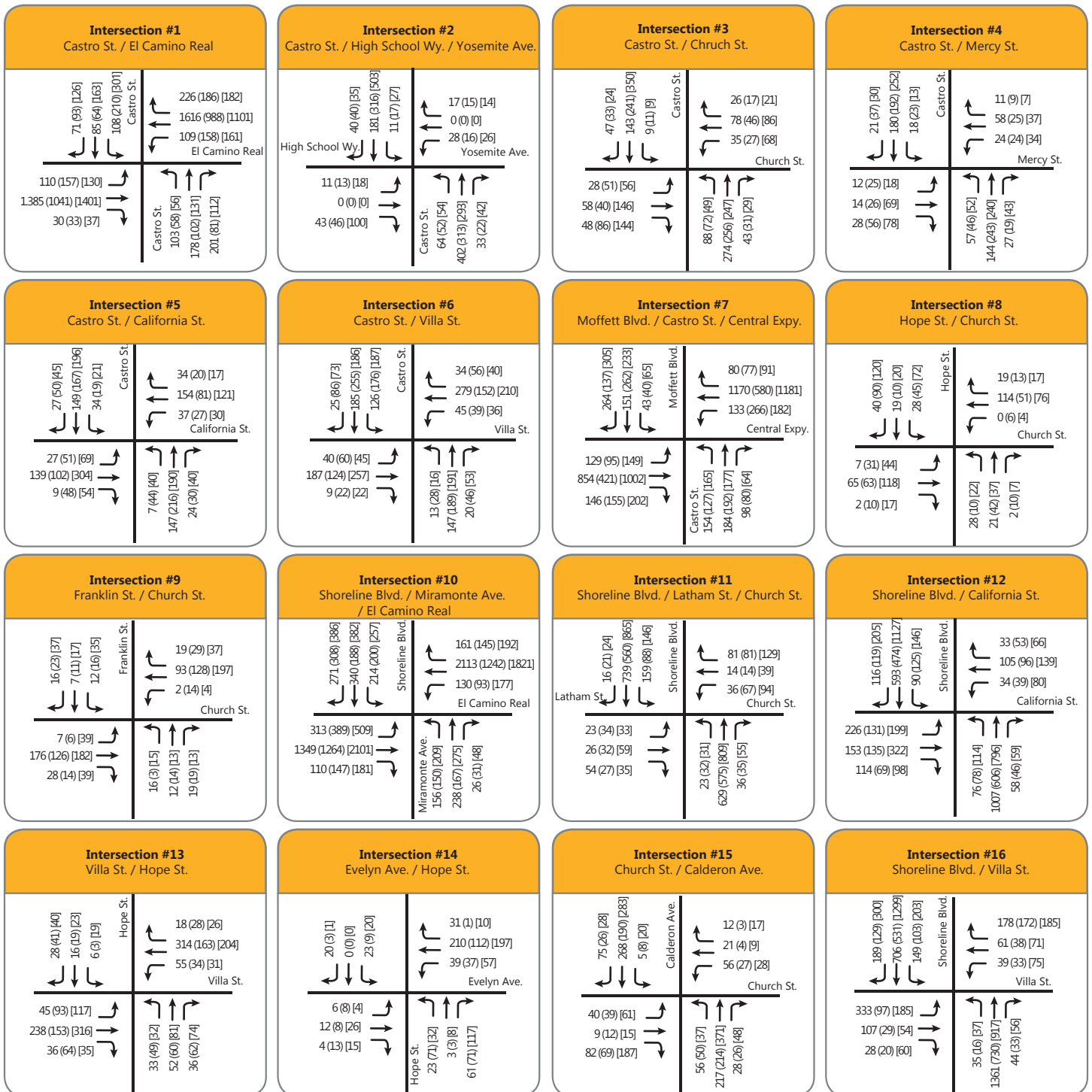
Figure 16. Baseline plus Project Conditions Peak Hour Traffic Volumes
