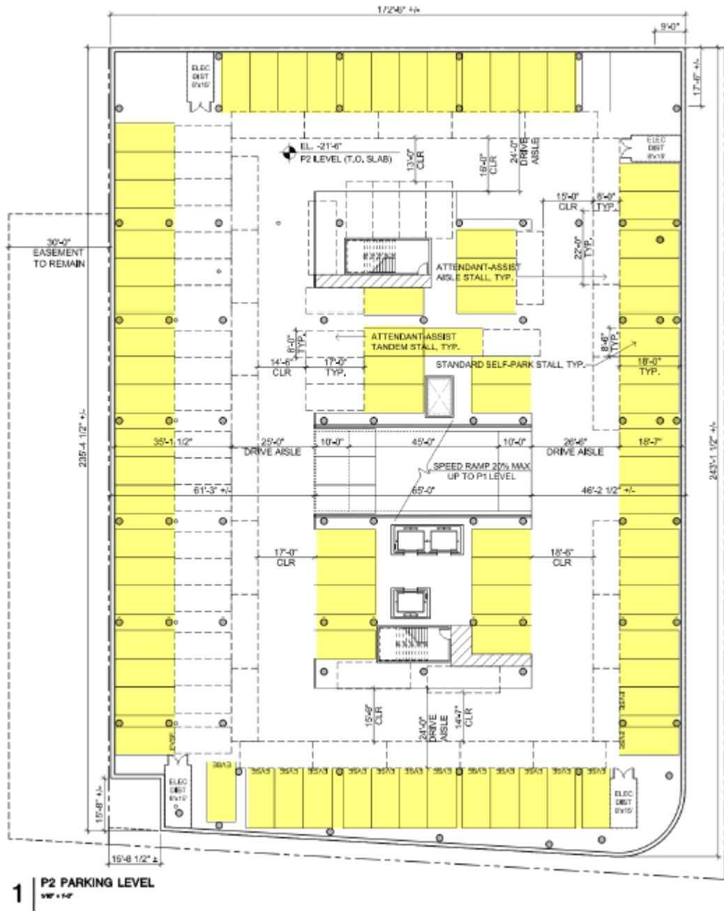
Figure 23. B2 Level Plan
