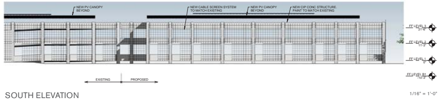
SOUTH ELEVATION
