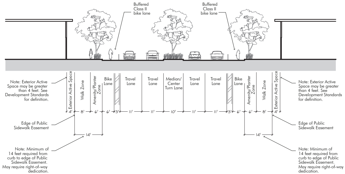
FIGURE 3-7 Showers Drive Section (C-C)
