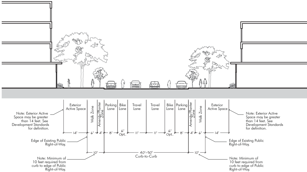
FIGURE 3-10 Typical Neighborhood Street Section (F-F)
