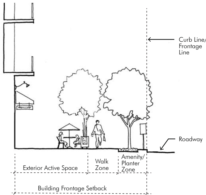
FIGURE 3-4 Sidewalk Diagram (Typical)
