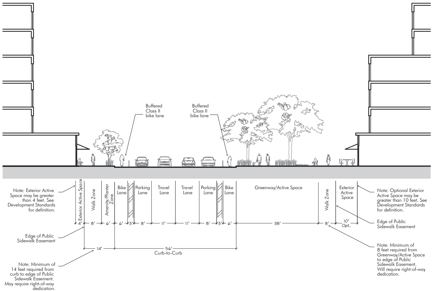
FIGURE 3-9 Pacchetti Greenway Section (E-E)
