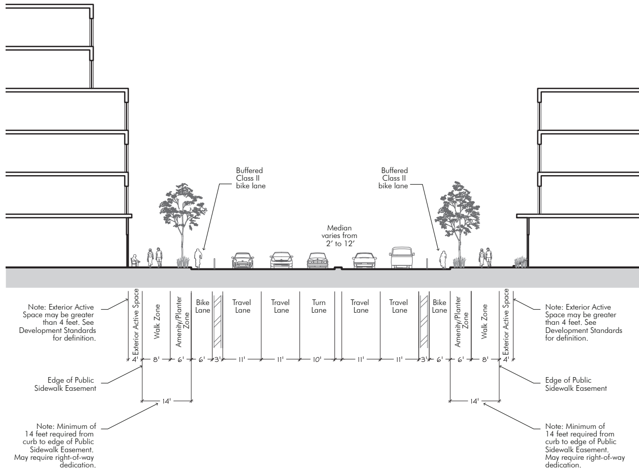
FIGURE 3-6 California Street Section (B-B)
