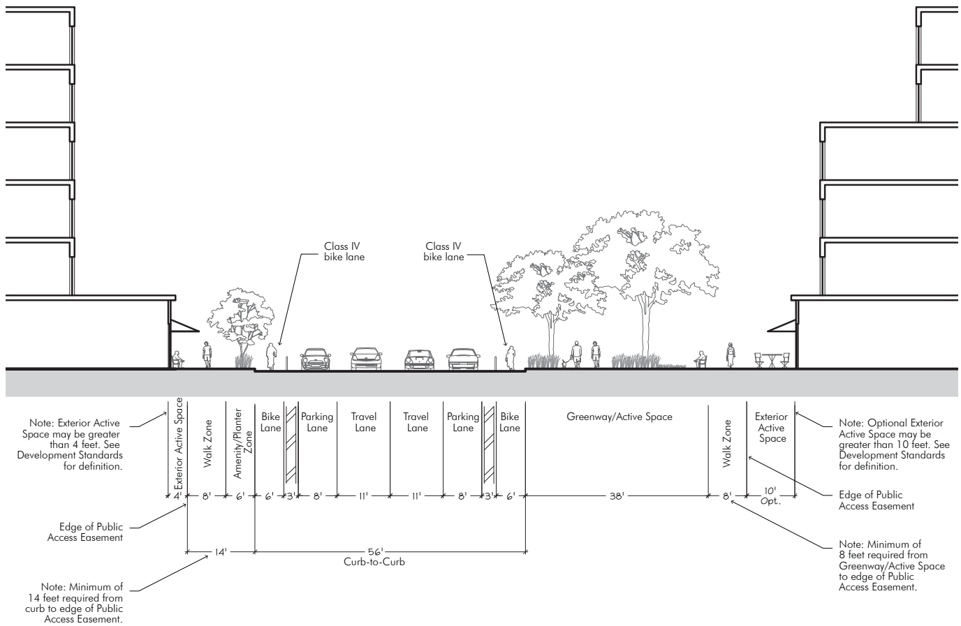
FIGURE 3-9 Pacchetti Greenway Section (E-E)
