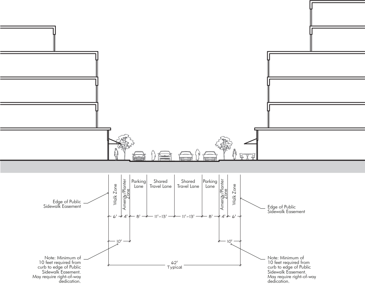
FIGURE 3-11 Typical Main Internal Street Section (G-G)
