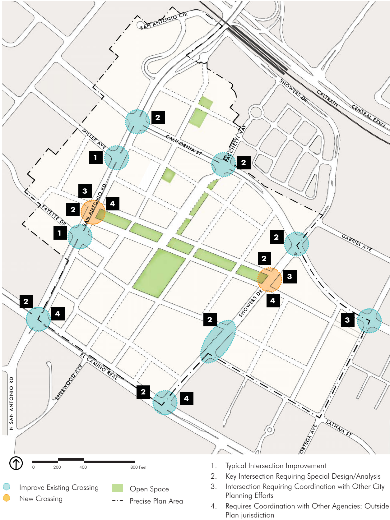
FIGURE 3-13 Key Intersections
