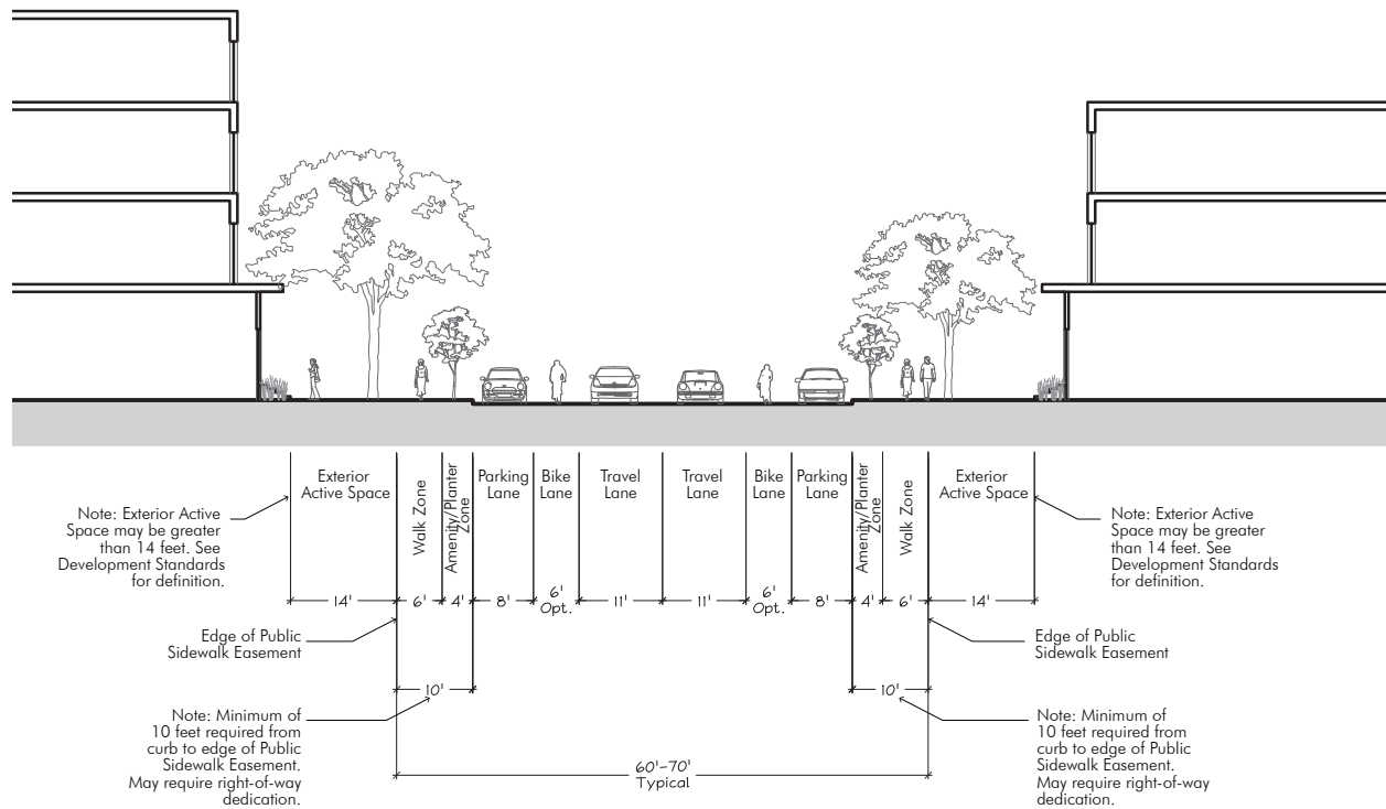
FIGURE 3-10 Typical Neighborhood Street Section (F-F)
