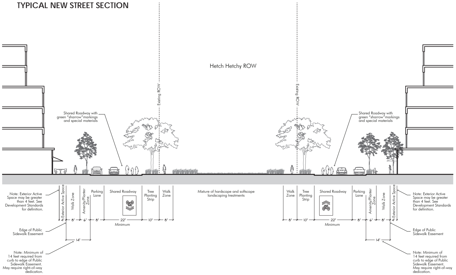
FIGURE 3-8 Hetch Hetchy Greenway Section (D-D)
