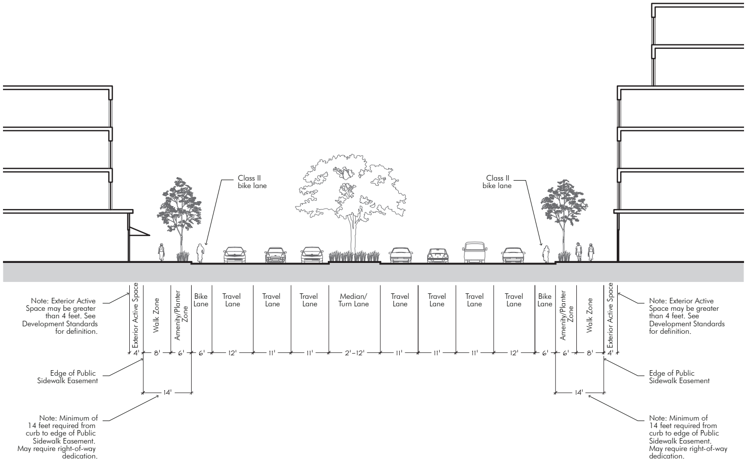
FIGURE 3-5 San Antonio Road Section (A-A)
