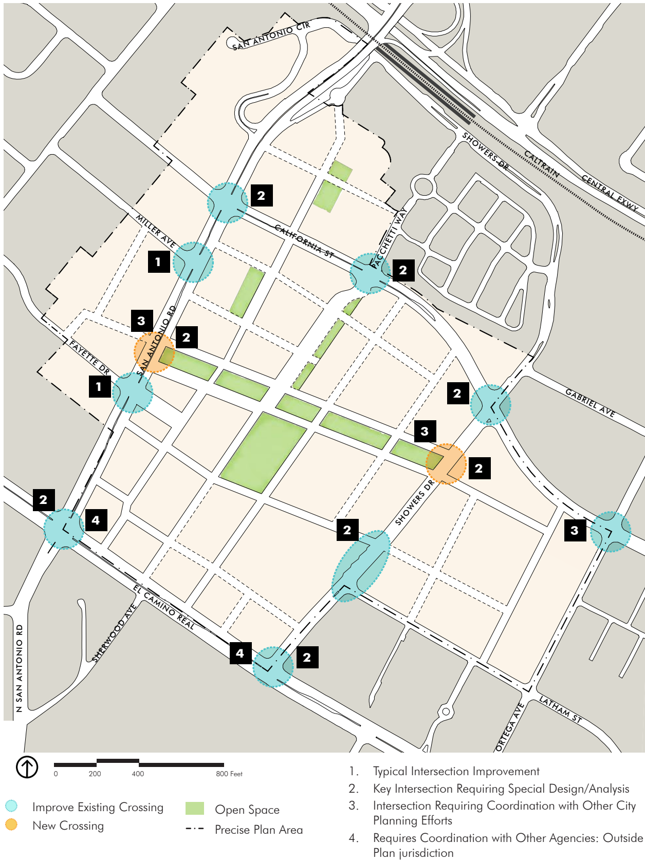
FIGURE 3-13 Key Intersections
