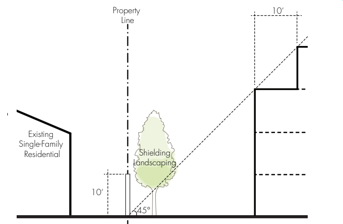
FIGURE 4-6 Single-Family Residential Transition
