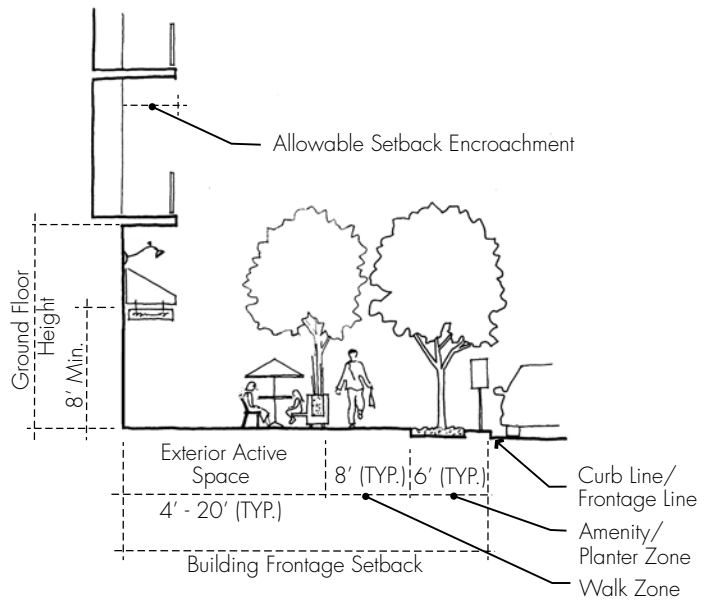
FIGURE 4-4 Frontage & Setback Standards
