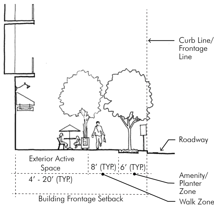
FIGURE 3-4 Sidewalk Diagram (Typical)
