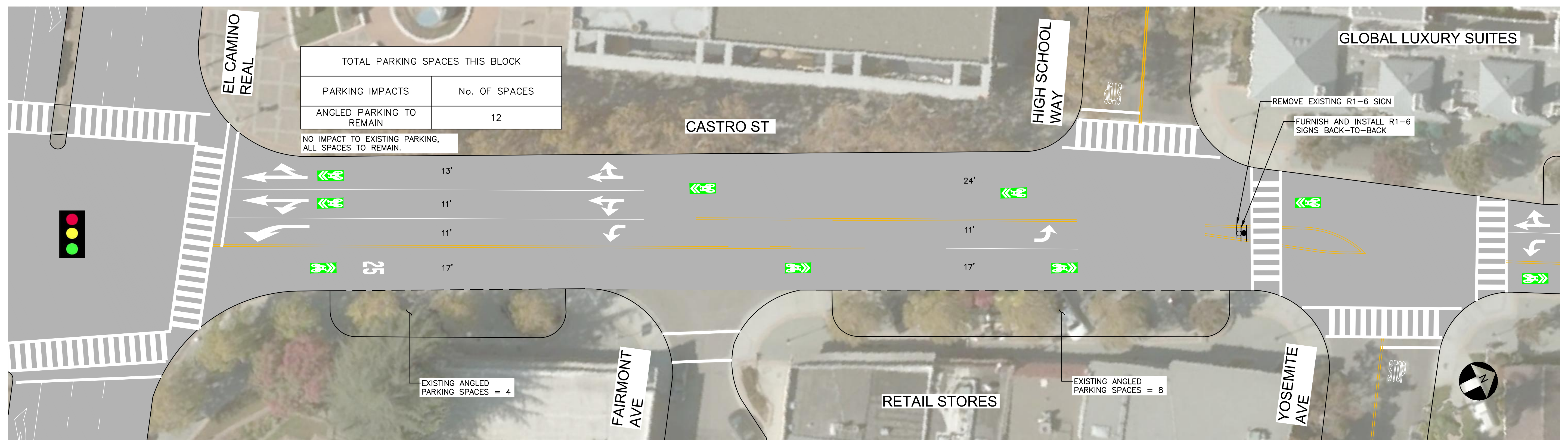
PROPOSED ROADWAY CONDITIONS
