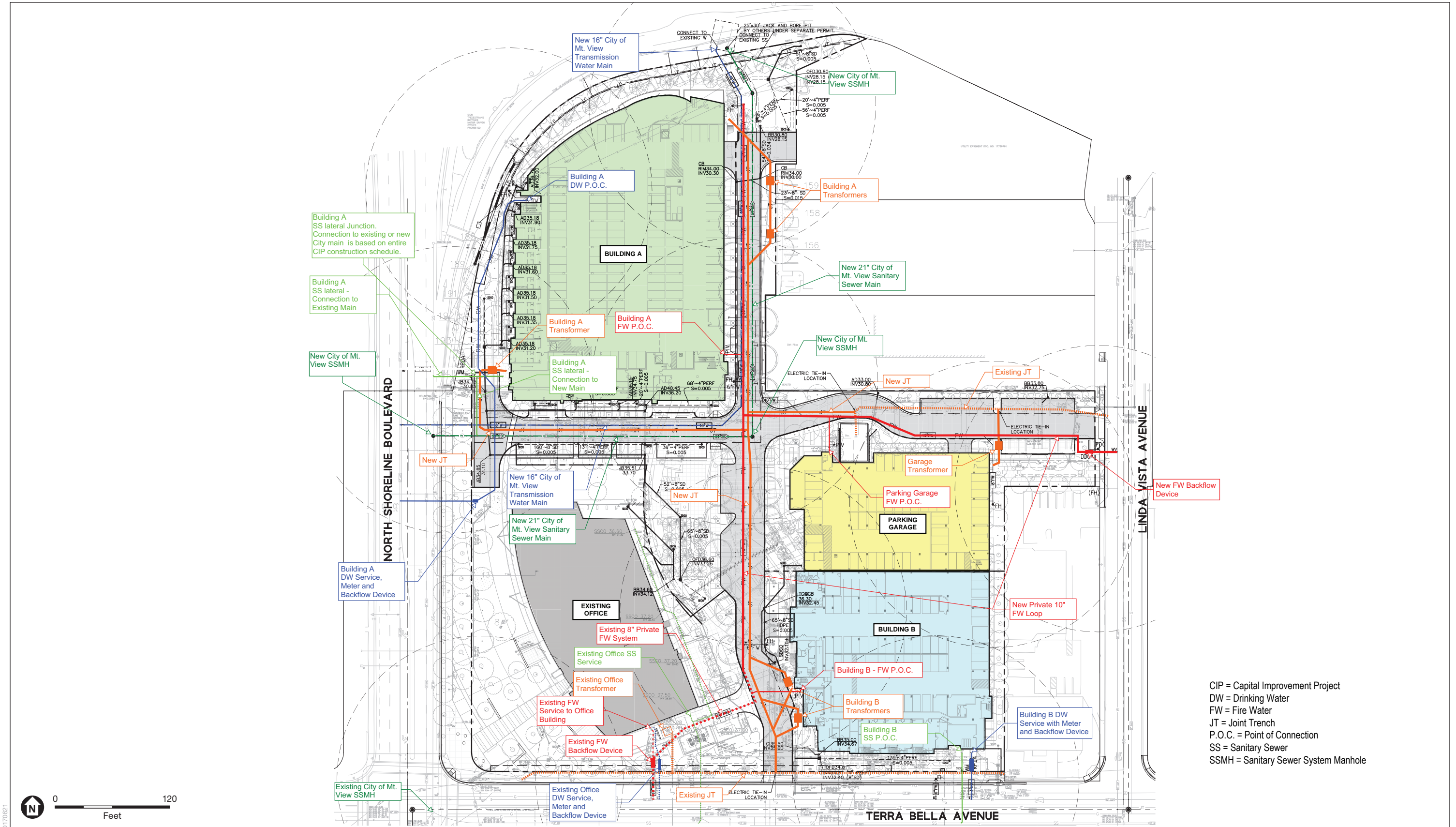
Figure 3-8 Proposed Utility Plan
