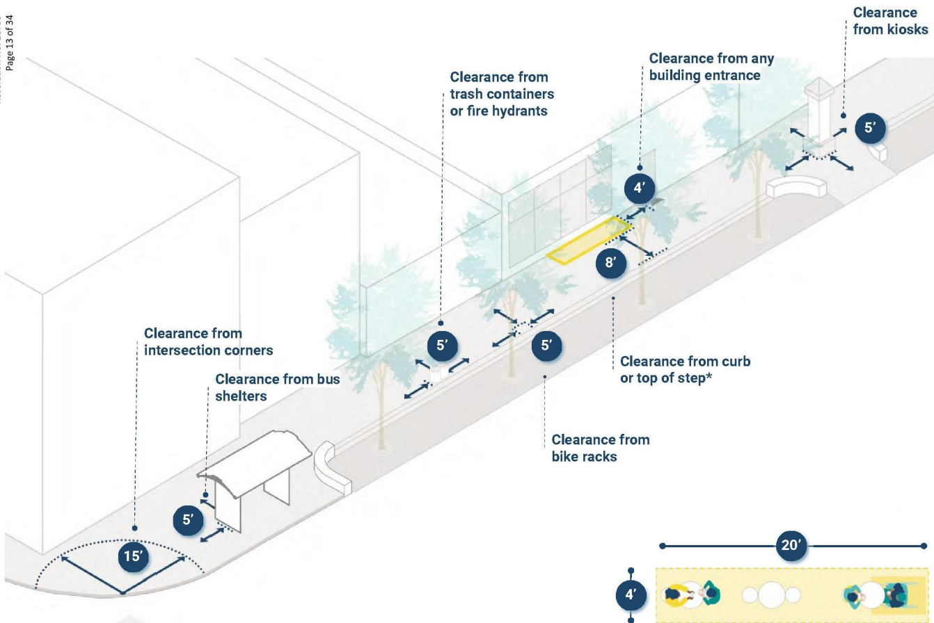
Figure 4: Sidewalk Patio Minimum Dimensions
