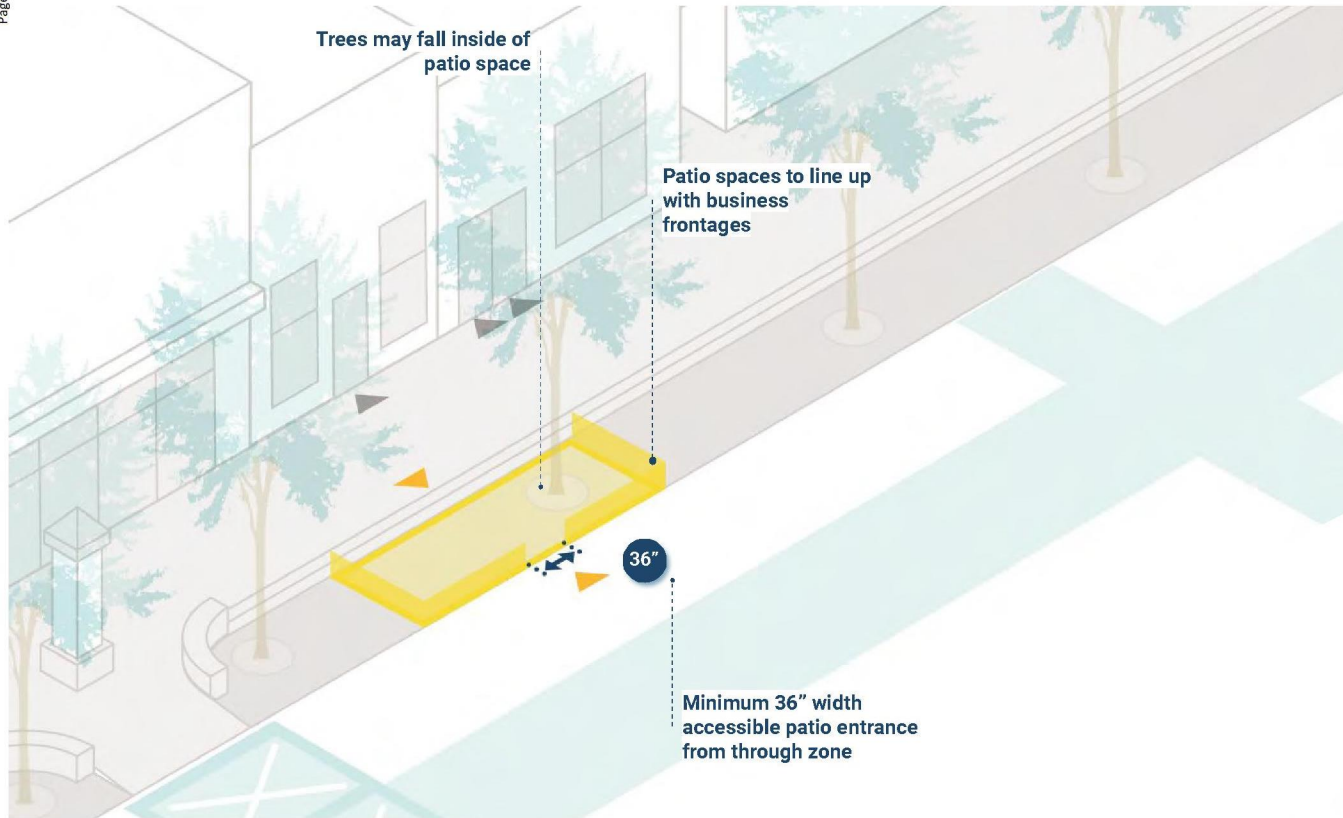
Figure 5: Patio Layout in 10' Program Zone
