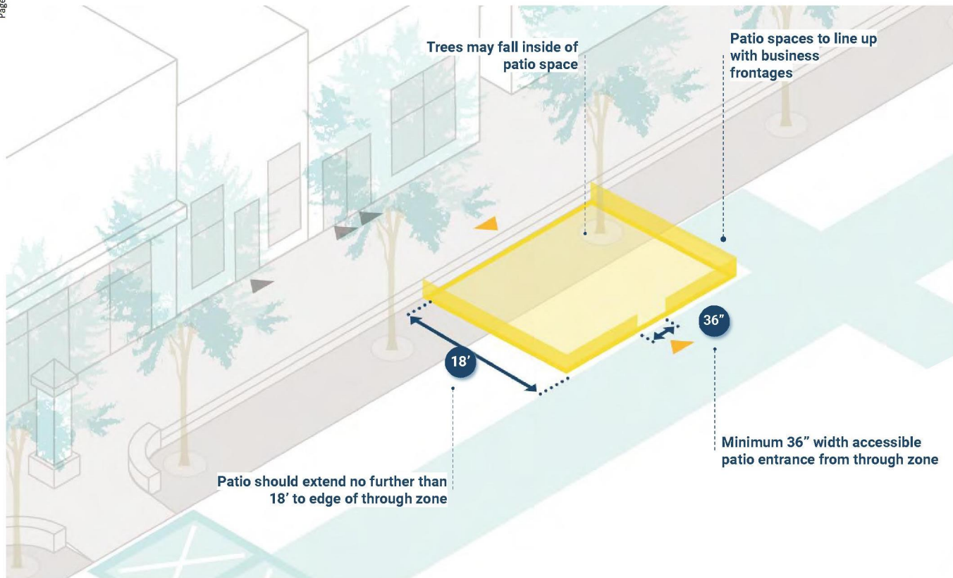
Figure 6: Patio Layout in 18' Program Zone
