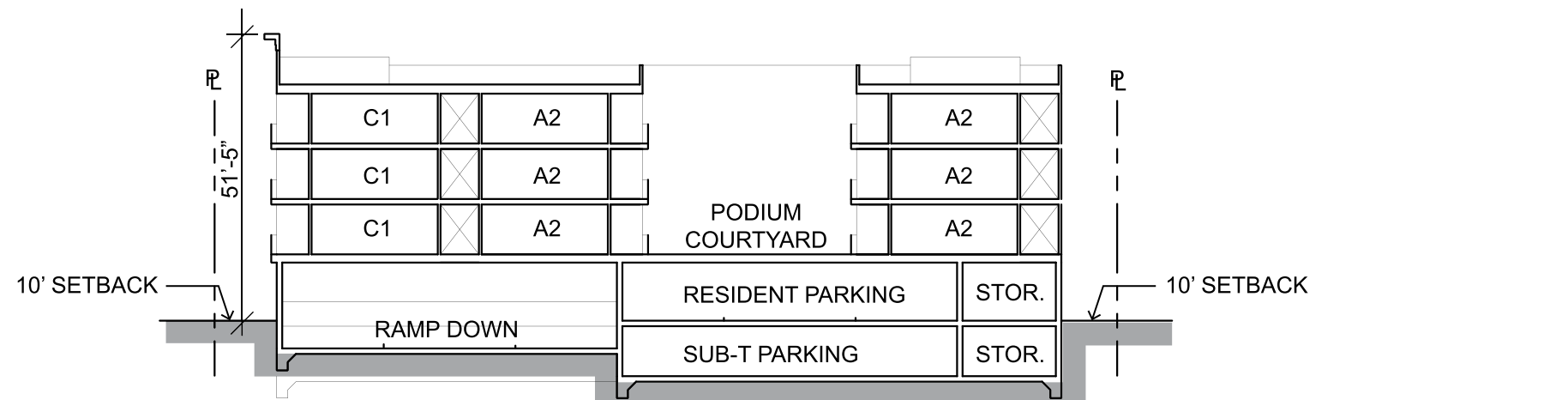
SITE SECTION C-C
