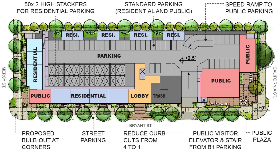
GROUND LEVEL / SITE PLAN (NOT TO SCALE)
