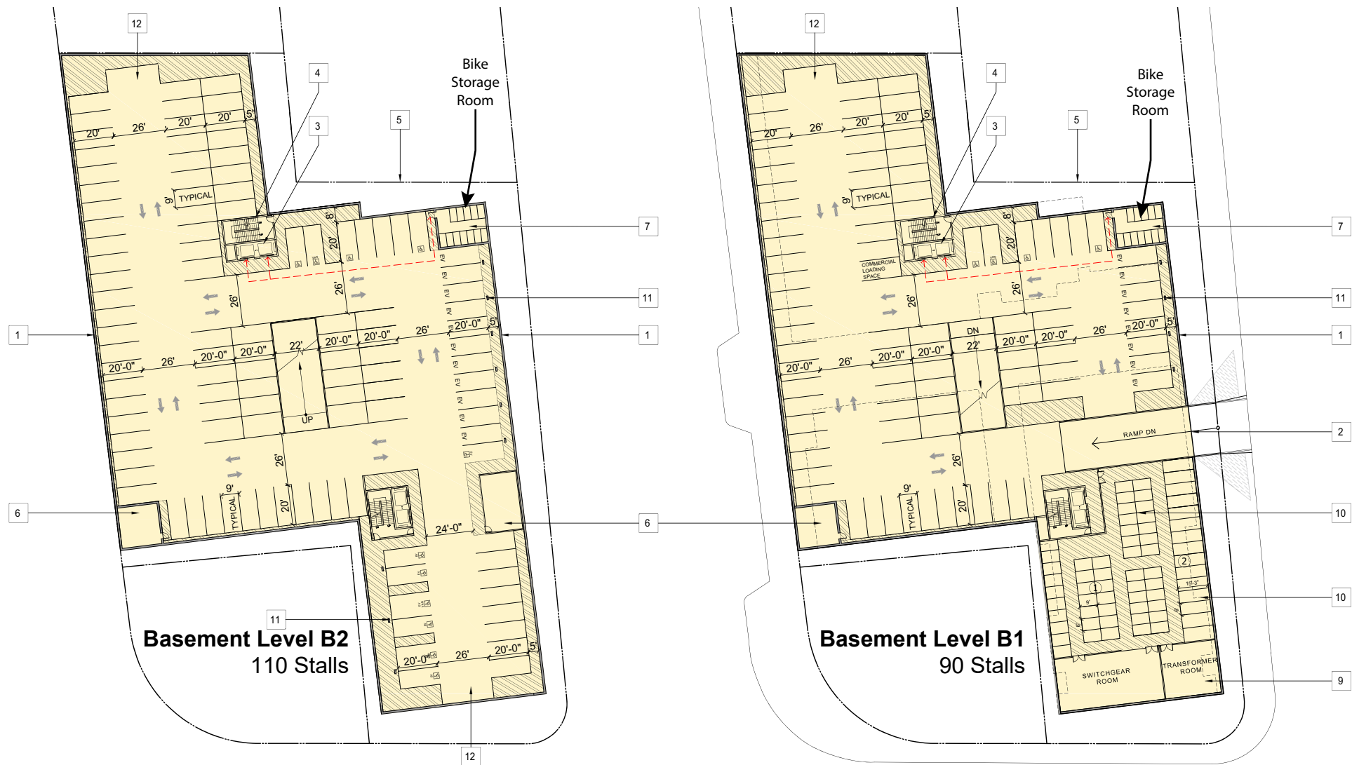
Figure 12 Parking Garage Plans
