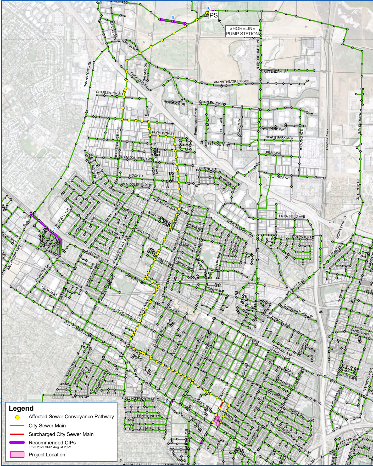
FIGURE 3: Peak Wet Weather Flow Sewer System Model
