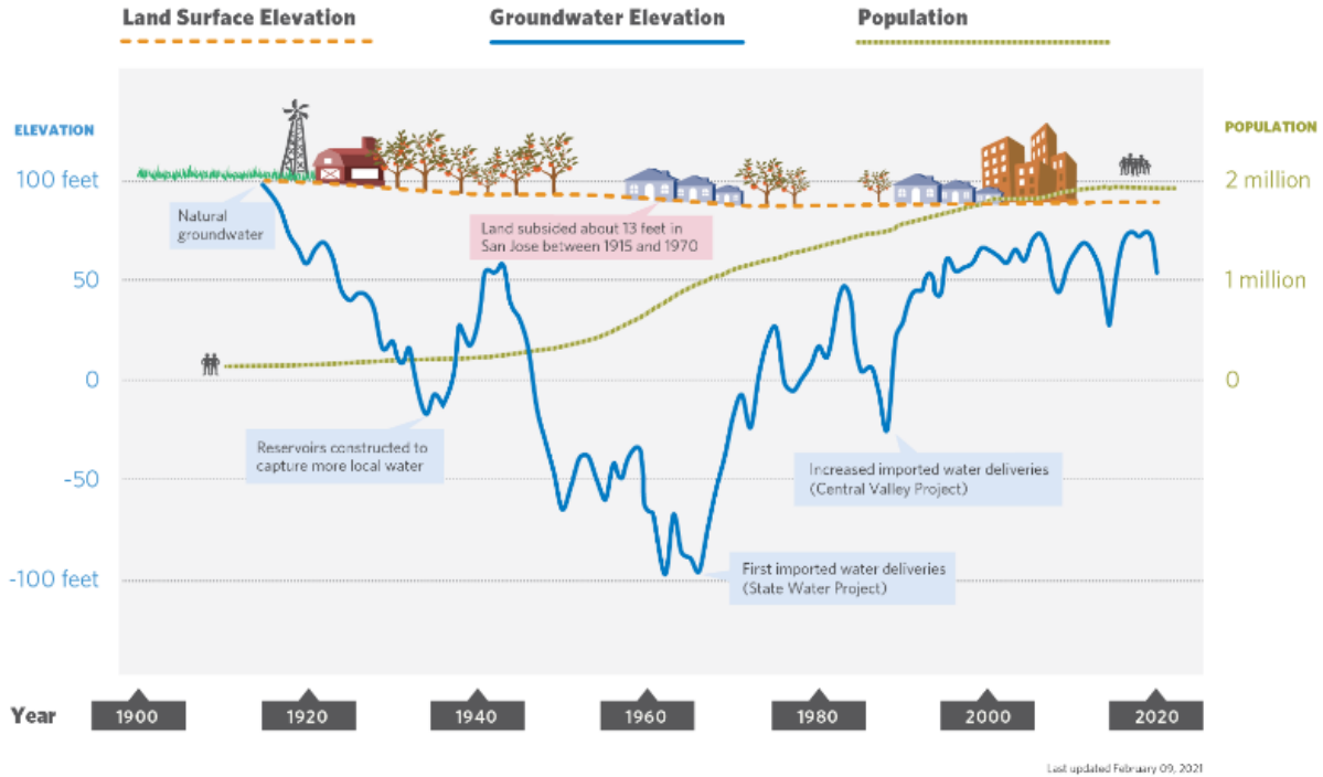
Figure 69: SCVWD Historic Groundwater Conditions 285
